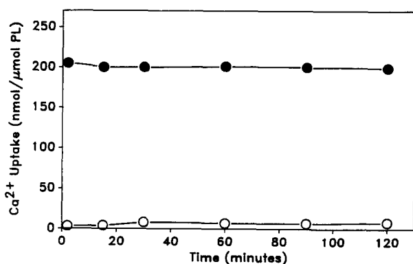
Fig. 7. The effect of internal buffer on A23187 (10 \mu\text{g/ml} ) mediated accumulation of \text{Ca}^{2+} in EPC LUVs (100 nm) in the absence of transmembrane pH gradient. 300 mM citrate (pH 7.4) (○), and 300 mM ethylenediaminetetraacetic acid (pH 7.4) (●). In both cases the external buffer was 300 mM sucrose, 20 mM Hepes (pH 7.4) and the phospholipid concentration 2.0 mM.
