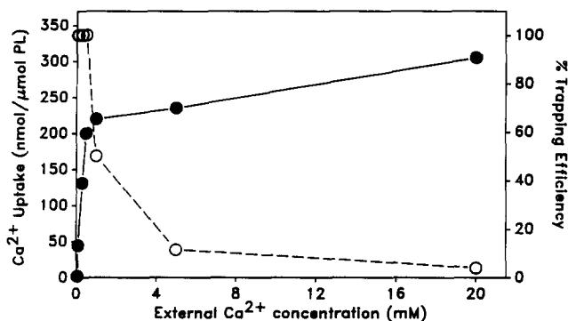
Fig. 4. The effect of initial extravesicular \text{Ca}^{2+} concentration on A23187 (10 \mu\text{g}/\text{ml} ) mediated \text{Ca}^{2+} uptake (●) and percentage trapping efficiency (○), into EPC LUVs (100 nm) experiencing a transmembrane pH gradient (300 mM sucrose, 20 mM Hepes (pH 7.4) in the external medium and 300 mM citrate (pH 4.0) in the internal medium). Measurements were made at two hours, and the phospholipid concentration was 2.0 mM.
