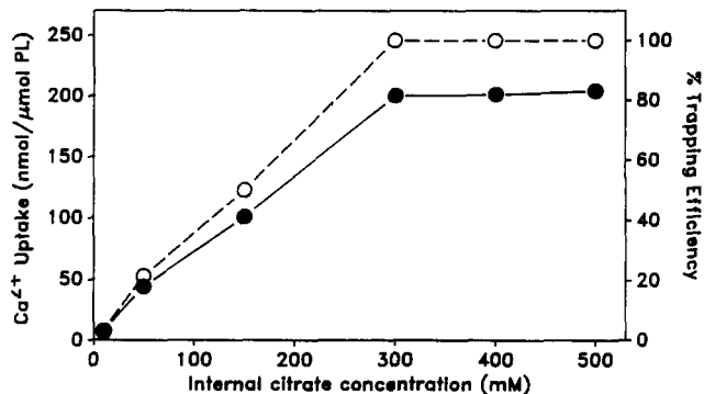
Fig. 5. The effect of internal citrate concentration on \text{Ca}^{2+} uptake (●) and percentage trapping efficiency (○) into EPC LUVs (100 nm) experiencing a transmembrane pH gradient (300 mM sucrose, 20 mM Hepes (pH 7.4) in the external medium and 300 mM citrate (pH 4.0) in the internal medium), in the presence of A23187 (10 \mu\text{g}/\text{ml} ) and 0.5 mM external \text{Ca}^{2+} . Measurements were made at two hours, and the phospholipid concentration was 2.0 mM.
